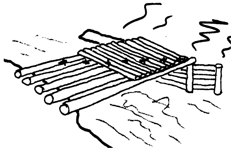
Figure 84. Slab bridge.
