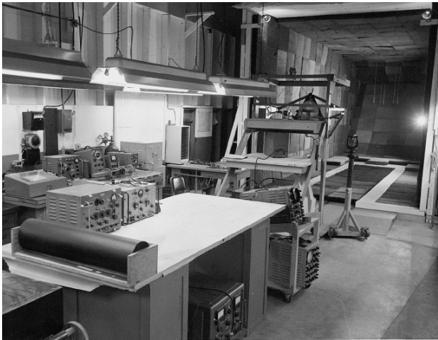
A rare look at Building 82, inside the fabled Lockheed Skunk Works, circa 1957. The world's first anechoic chamber can be seen at the far rear of the room. Shoe-sized models of the CIA's spy planes would be hung from the ceiling and tested. (Collection of Lockheed Martin)
