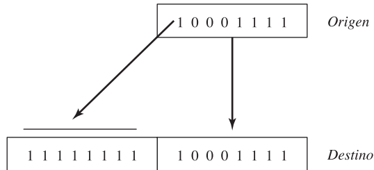
FIGURA 4-2 Diagrama de MOVSX ax,10001111b.
