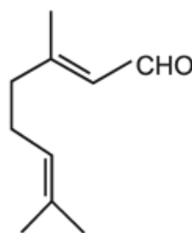
Geranial
