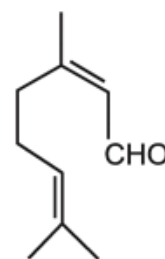
Neral
